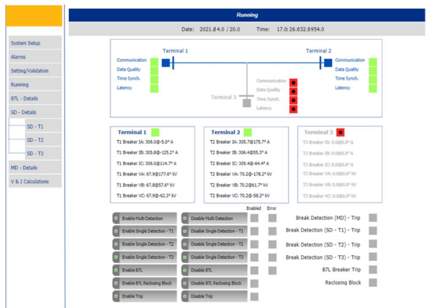
Figure 15: Example PMU TFCP and 87LN protection scheme operating display on PC
