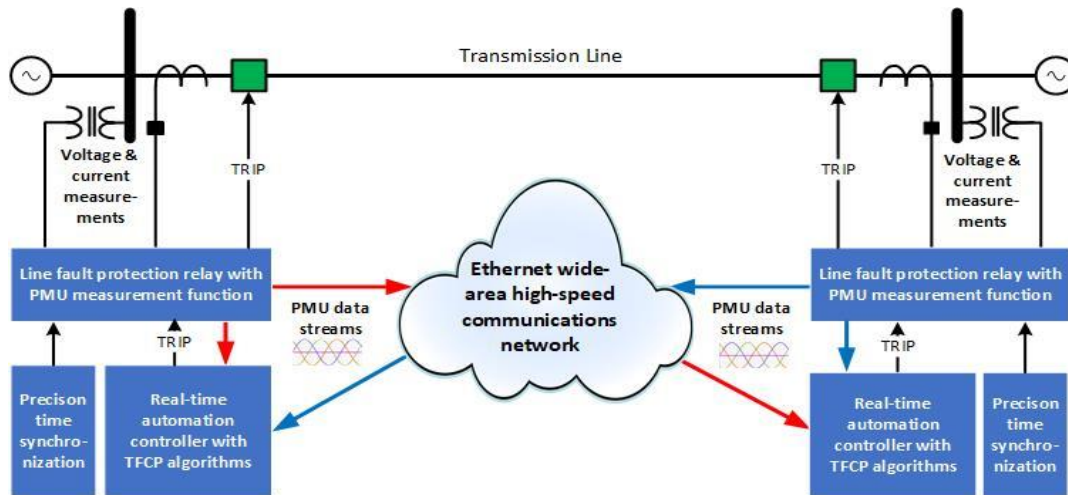
Figure 8: Components of a transmission falling conductor protection (TFCP) system
