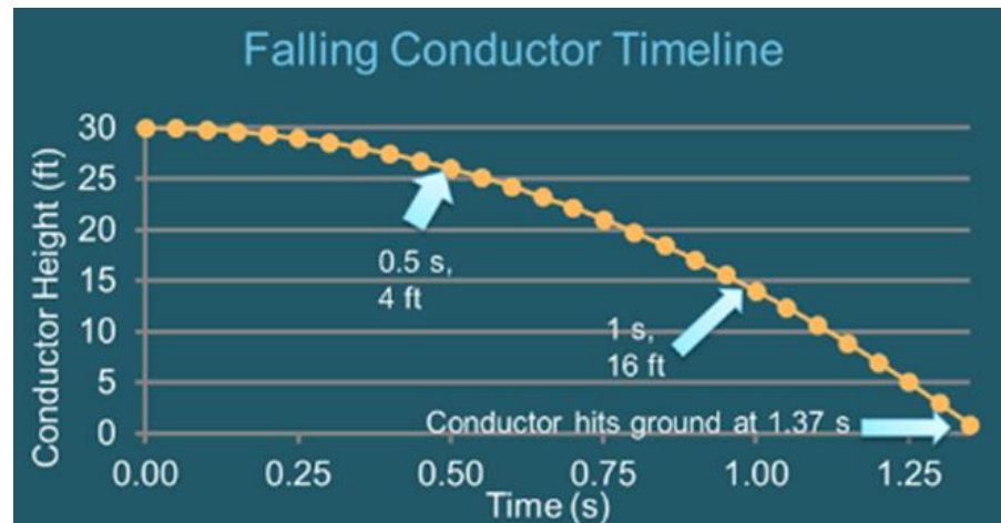
Figure 2: Distribution falling conductor operational timing
