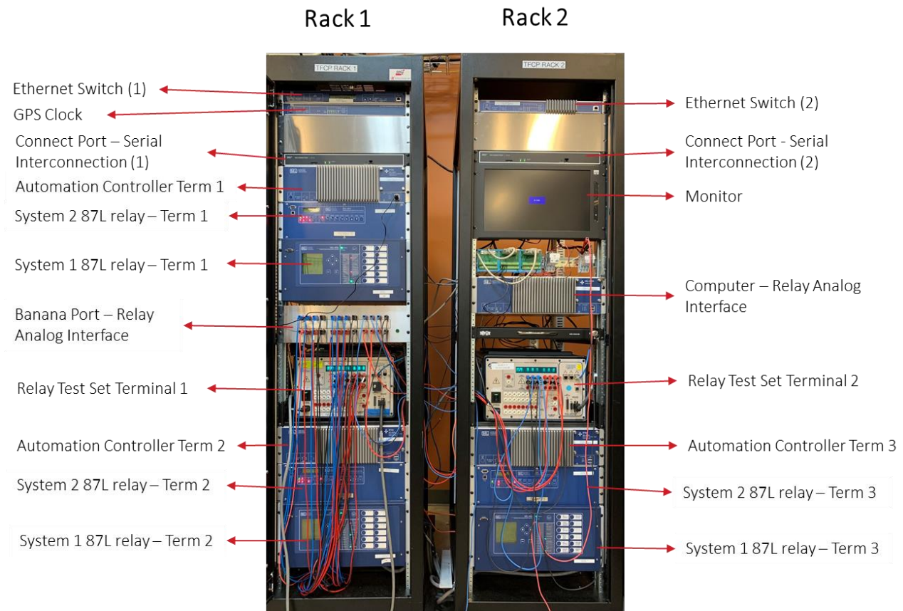
Figure 12: RTDS equipment rack configurations for TFCP and 87LN testing
