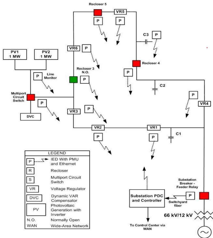
Figure 3: FCP circuit IED deployment example
