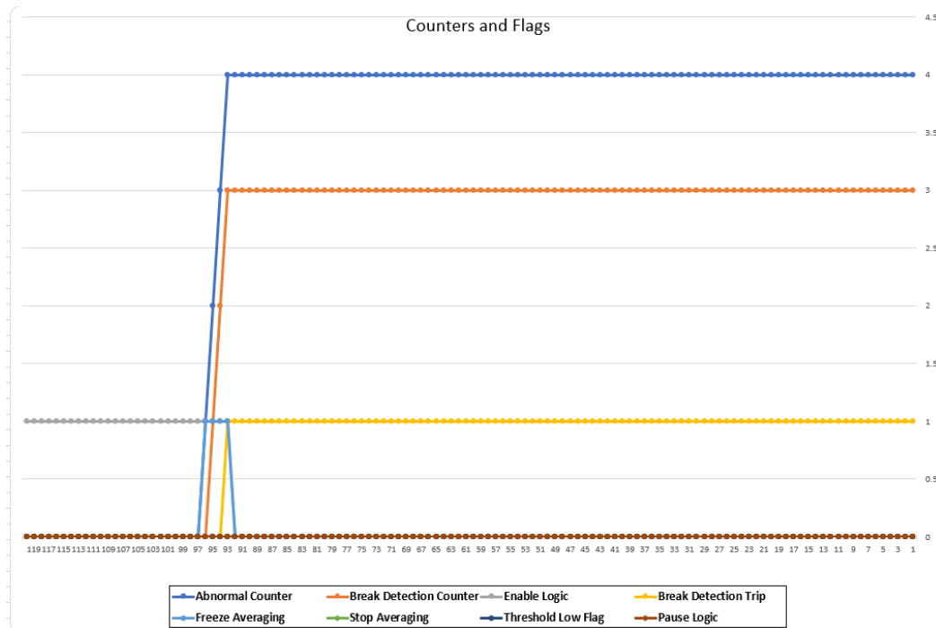
Figure 10b: Break detection in Phase A – counters and flags
