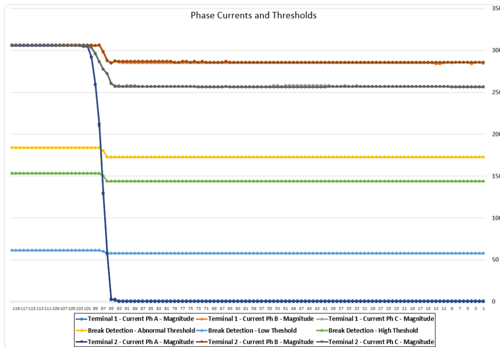
Figure 10a: Break detection in Phase A – phase currents and thresholds
