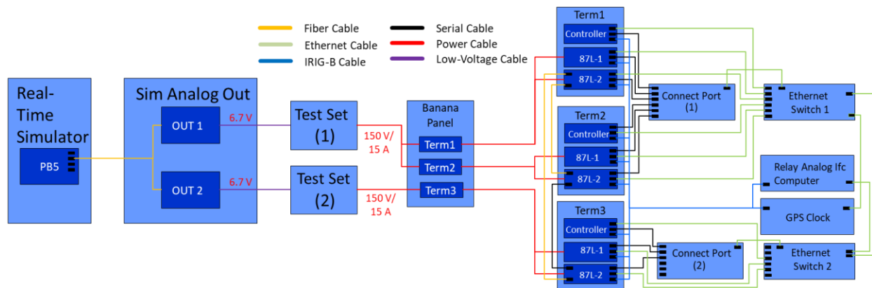
Figure 13: Connection of RTDS and test rack equipment for TFCP tests and evaluation
