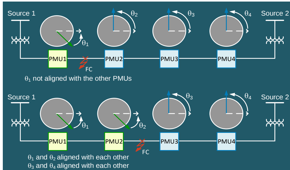
Figure 6: Conductor break location from relationships of V_2/V_0 phase angles along circuit
