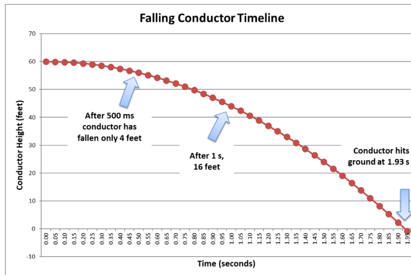
Figure 9: Transmission falling conductor operational timing
