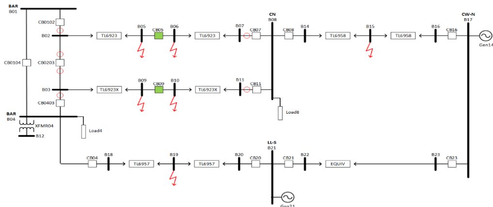
Figure 14: Simplified illustration of RTDS model of 69 kV transmission system with simulated breaks and high impedance faults
