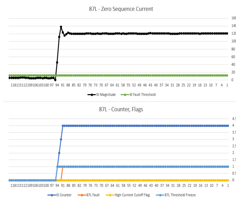
Figure 17: Example 87LN fault test result
