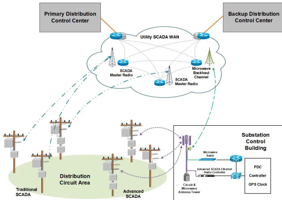
Figure 4: FCP radio communications architecture
