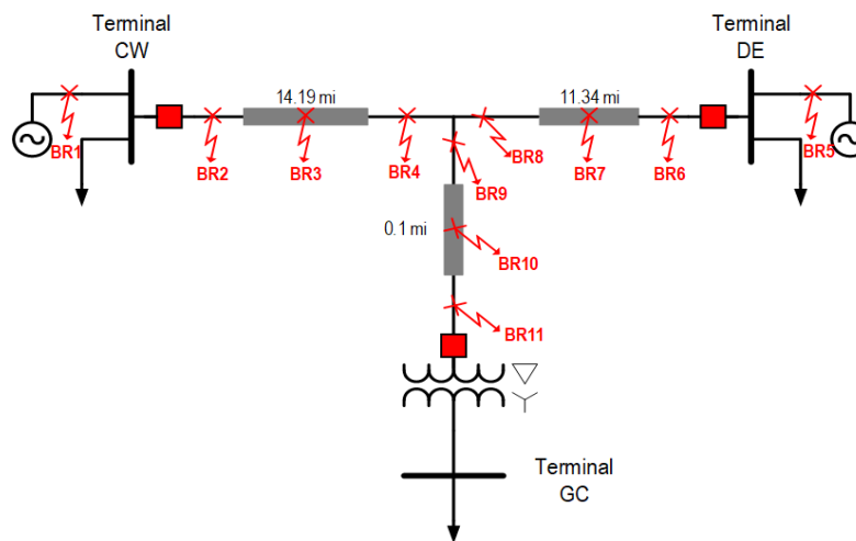
Figure 18: RTDS parallel test of PMU-based TFCP and relay internal logic for FCP on SDG&E field test line model
