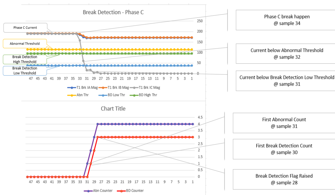
Figure 16: Example TFCP test result
