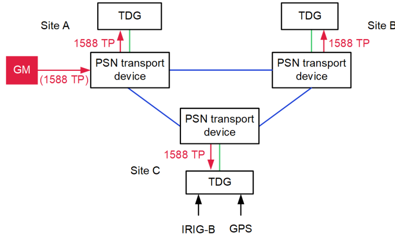
Figure 5. Validation Configuration for Network Model B.
