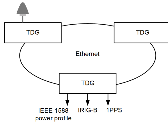
Figure 2. Network Model A
