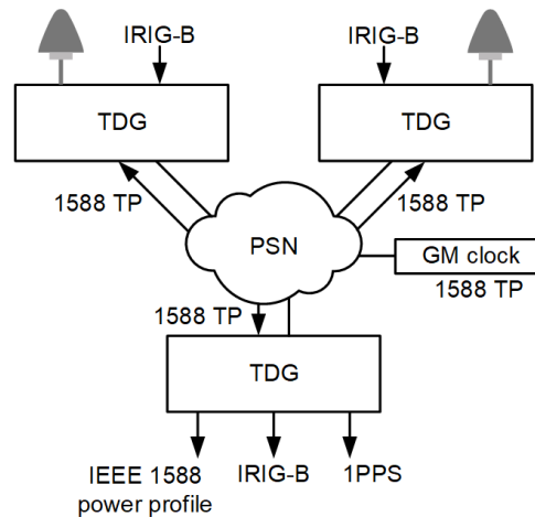
Figure 3. Network Model B
