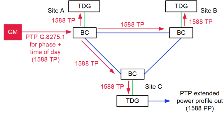
Figure 4. PTP Flows Through Network Model B
