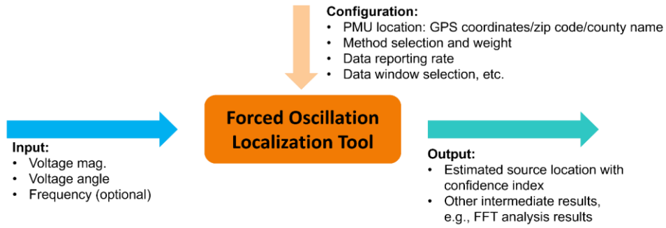
Figure 2. Diagram of the developed Forced Oscillation Localization Tool (FOLT)
