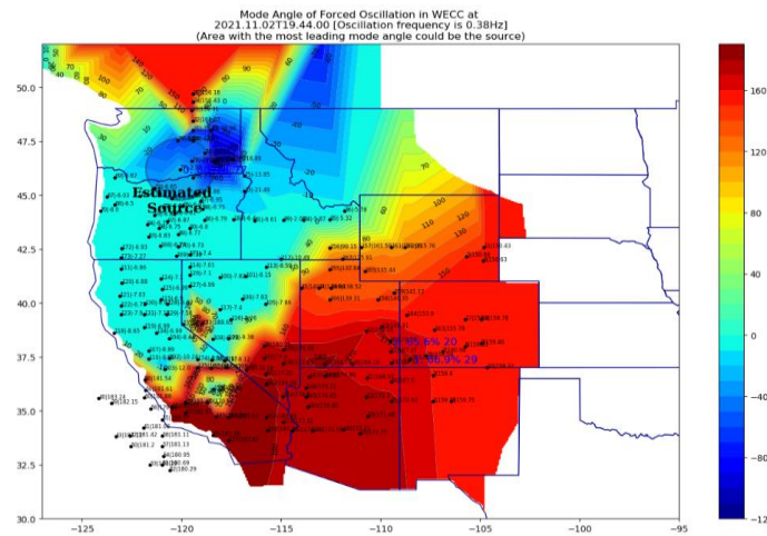
(c) Oscillation mode angle-based method
