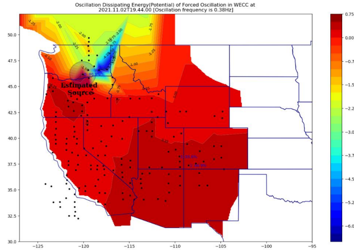
(a) Dissipating potential-based method
