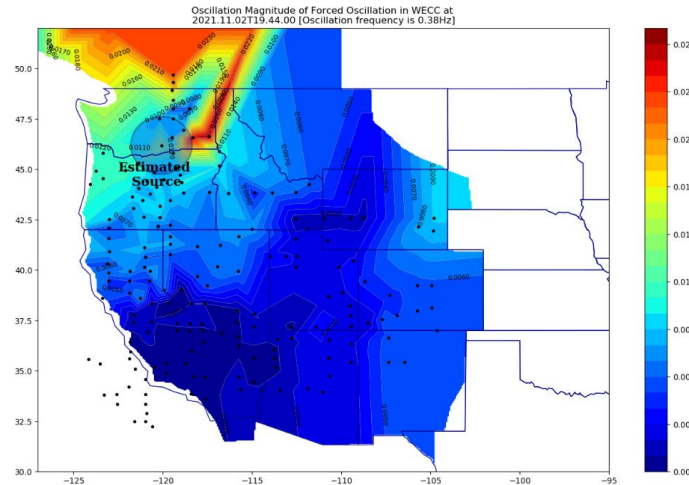
(b) Oscillation magnitude-based method
