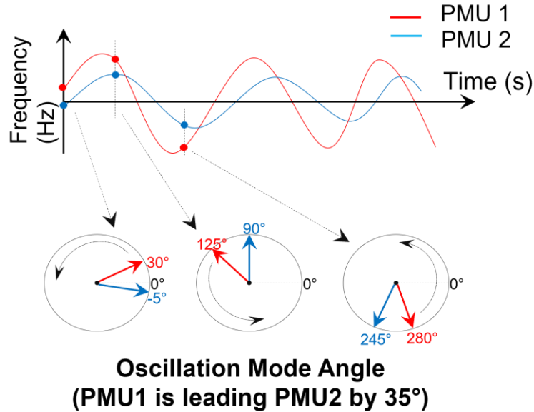
Figure 1. Oscillation mode angle between two PMUs
