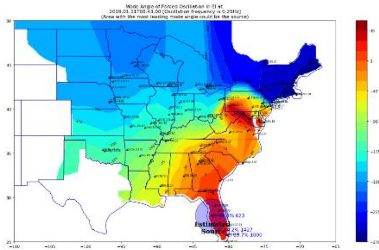
(c) Oscillation mode angle-based method
