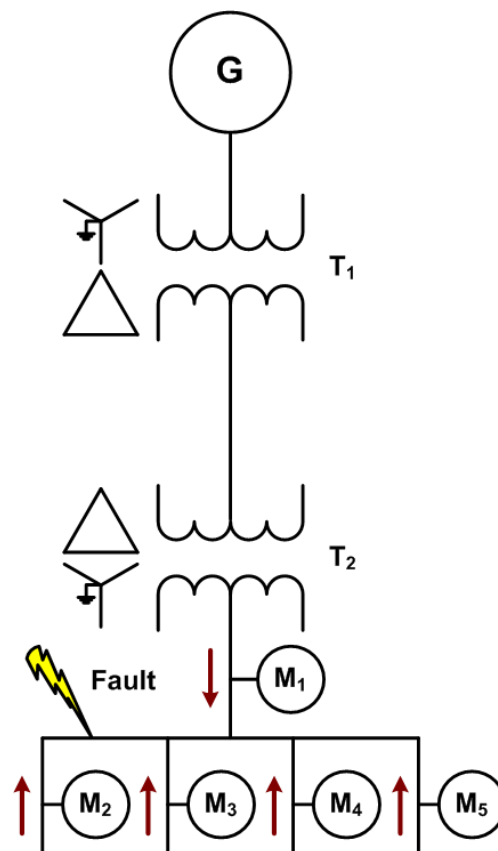
Figure 1: Simple One-Line Diagram Showing Multiple Monitoring Devices being used to Approximate a Disturbance Source.
