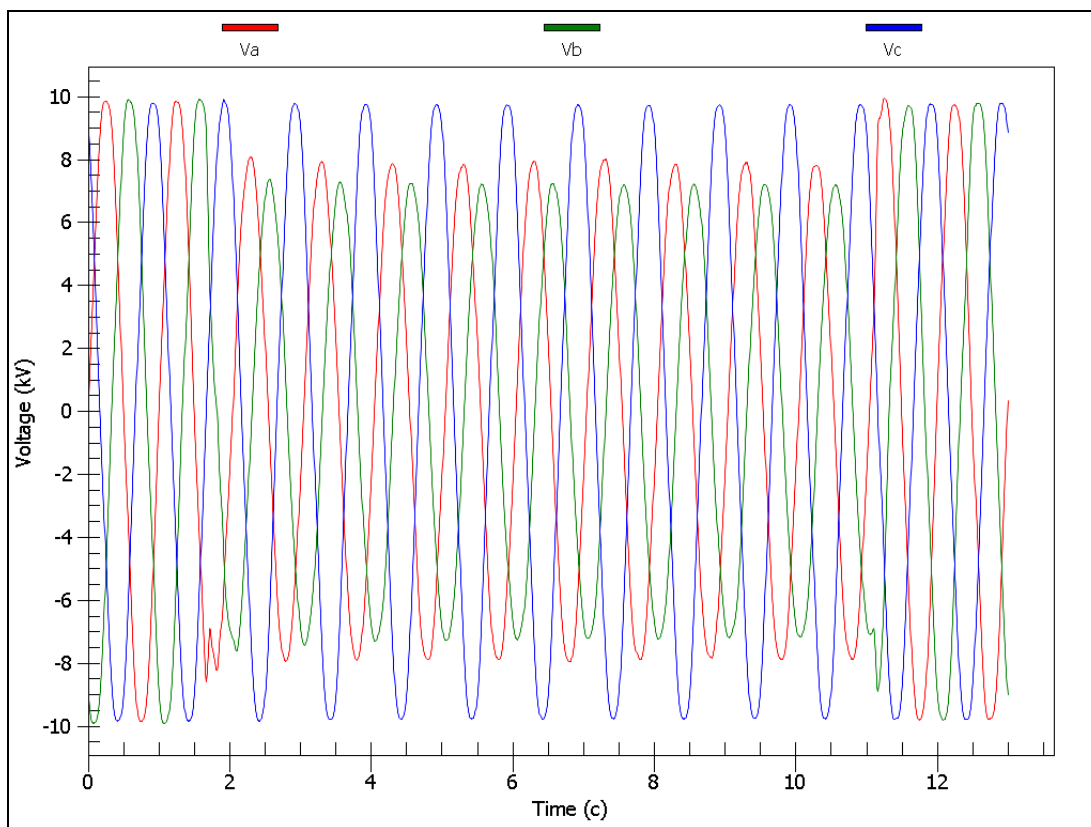
Figure 2: Voltage Sag Example: Three-Phase Voltage Waveform Samples
