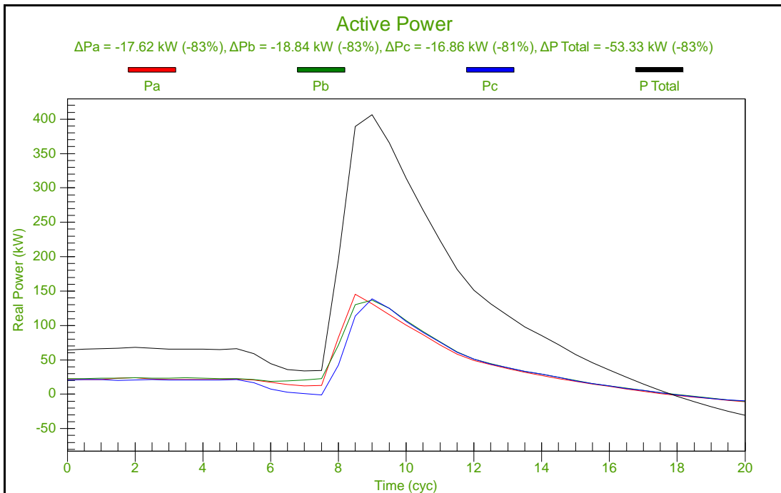
Figure 7: Active Power from Voltage Sag in Figure 5
