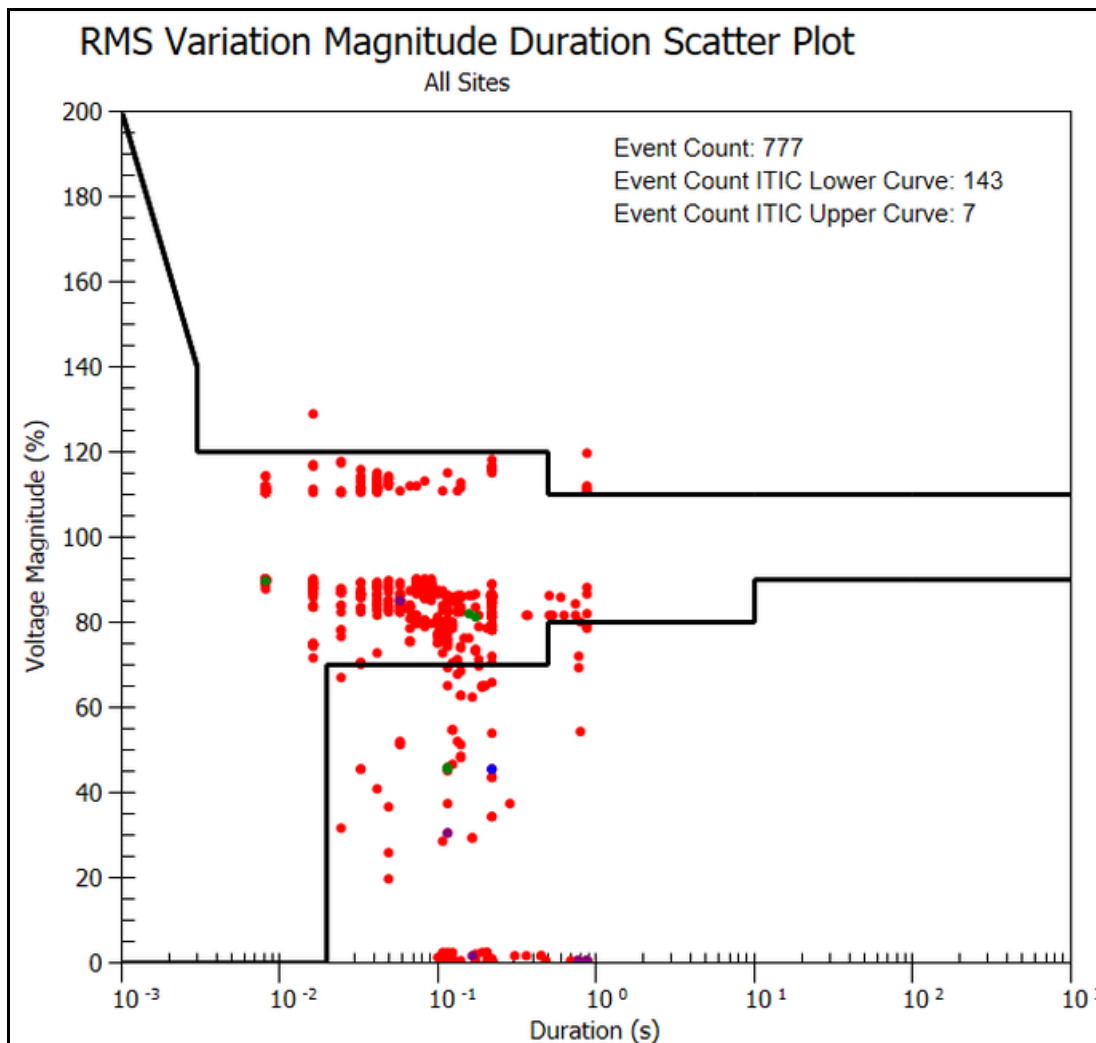
Figure 8: RMS Variation Magnitude-Duration Scatter Plot Displaying Voltage Sags with Load Loss
