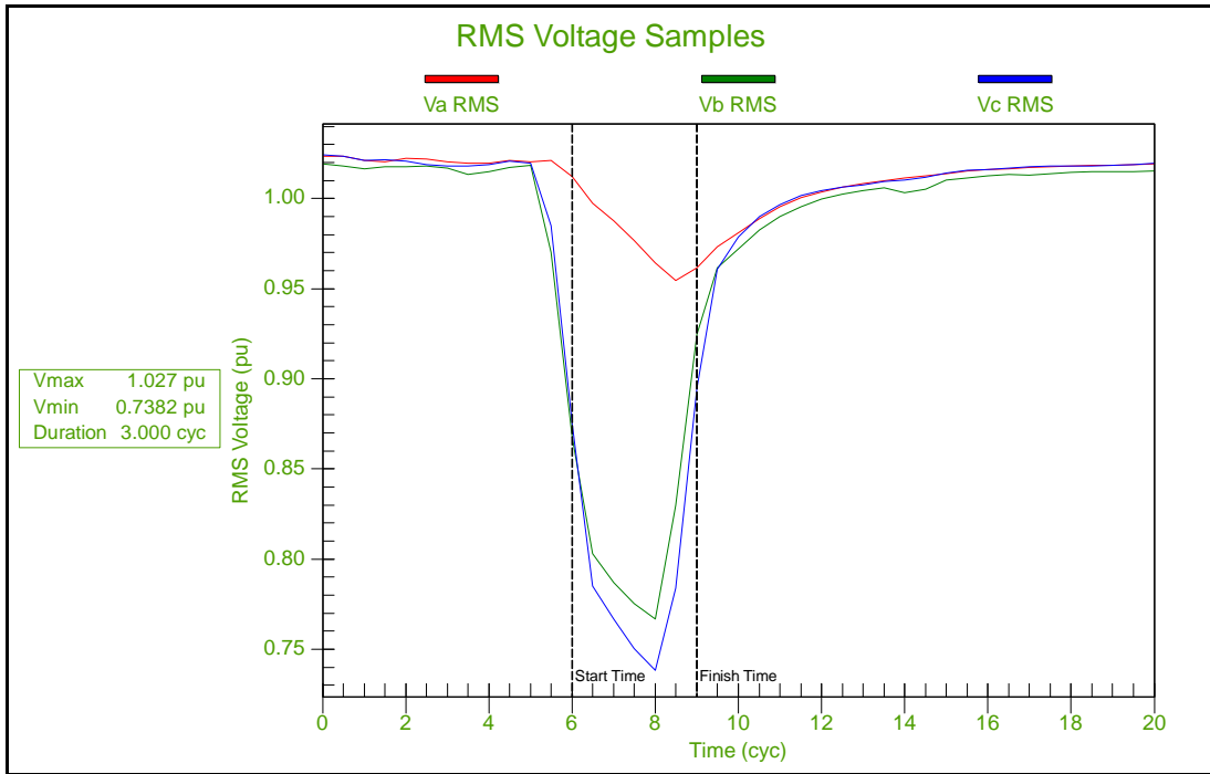
Figure 6: First 20 Cycles of RMS Voltage from Voltage Sag for Waveforms Samples in Figure 5
