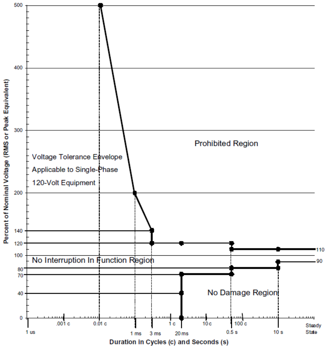
Figure 4: Information Technology Industry Curve (ITIC Curve)
