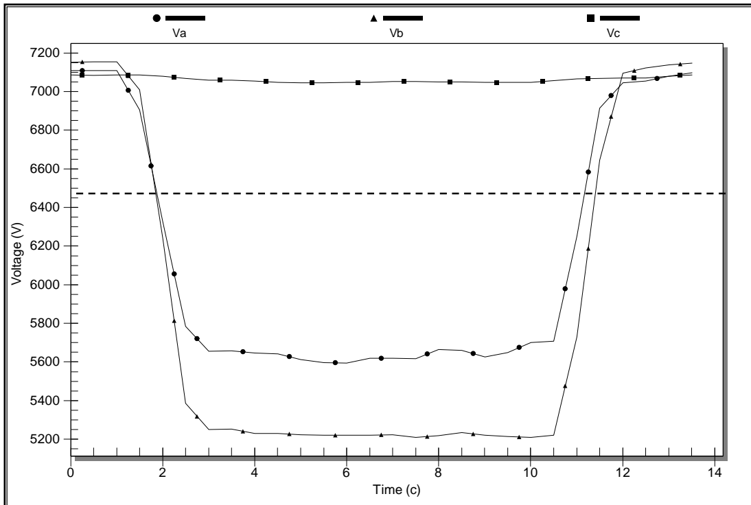
Figure 3: Voltage Sag Example: Three-Phase Voltage RMS Samples with Sag Threshold
