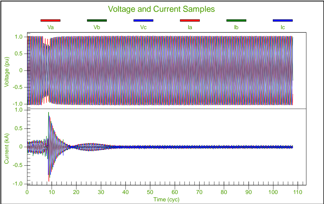
Figure 5: Instantaneous Waveform Capture of Voltage Sag
