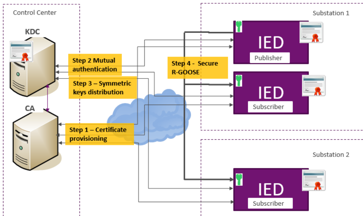
Figure 6: Key Distribution for Secure M2M Communications
