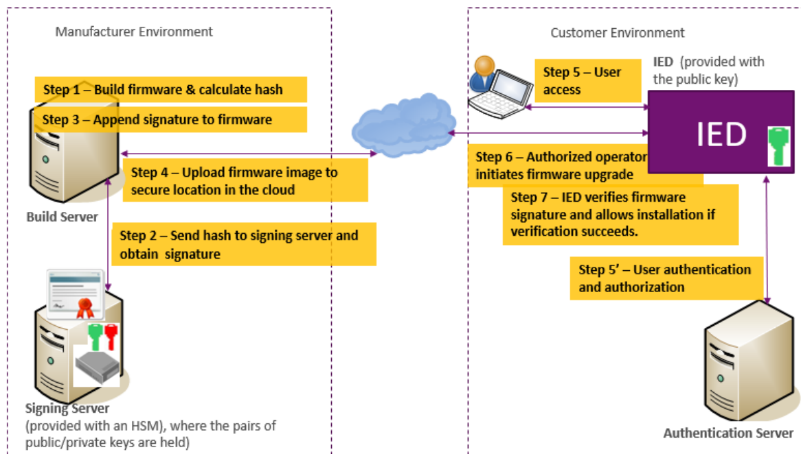
Figure 4: Firmware signing and verification procedure
