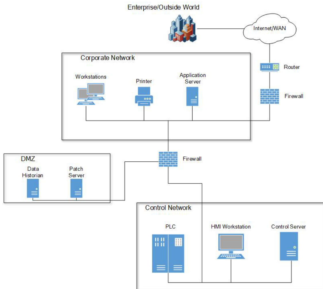
Figure 2 – DMZ Network to support Control Network (from NIST SP 800-82 R2)
