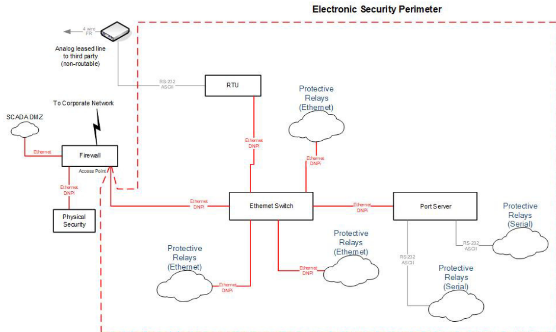
Figure 1 – Simple Substation Network Diagram
