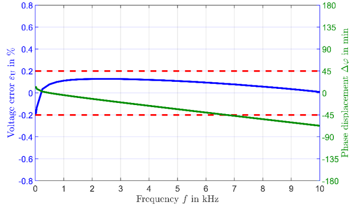
Figure 6: Frequency response of voltage accuracy \varepsilon_U(f) (blue) and phase displacement \Delta\phi(f) (green) of an AIS RC-divider type ROF 420. [10]
