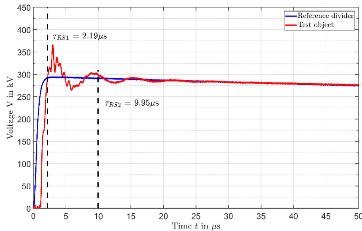
Figure 10: Step response behaviour – AIS type RGF 320DC
