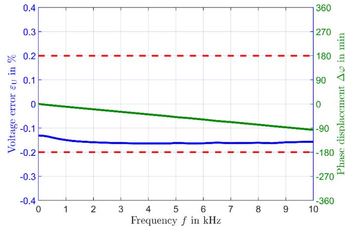
Figure 7: Frequency response of voltage accuracy \varepsilon_U(f) (blue) and phase displacement \Delta\phi(f) (green) of an GIS RC-divider type RGK 500DC.
