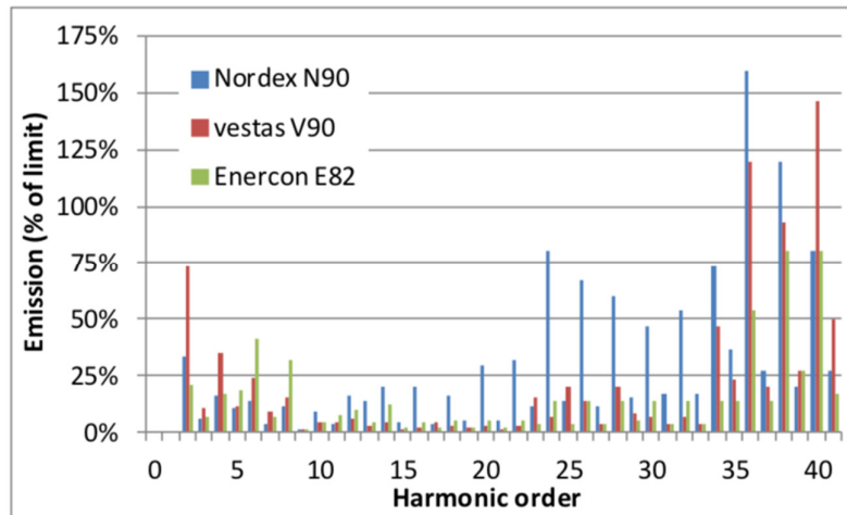
Figure 1 – Harmonic Emission Limits according to IEEE 519 limits
