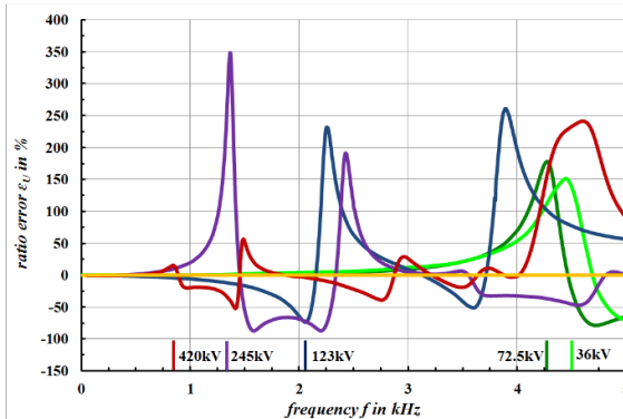
Figure 3: Frequency response of \varepsilon_U(f) for 36kV-VT(light green), 72.5kV-VT(dark green), 123kV-VT(blue), 245kV-VT(purple), 420kV-CTVT(red) and 420kV-RC-divider (yellow), as measured at PFIFFNER
