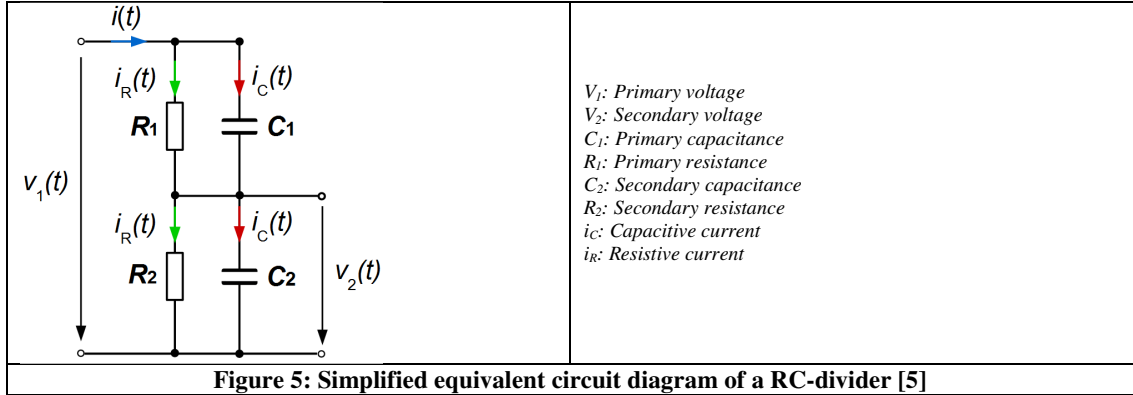
Figure 5: Simplified equivalent circuit diagram of a RC-divider [5]
