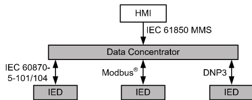
Figure 3 Common HMI communications flow
