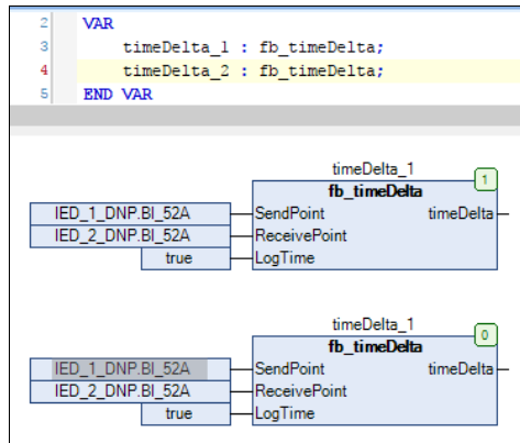
Figure 7 Time delta calculation in CFC
