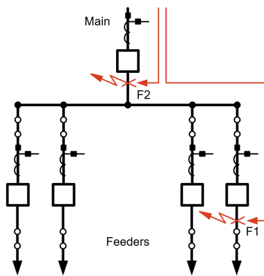
Figure 2 Fast bus tripping scheme
