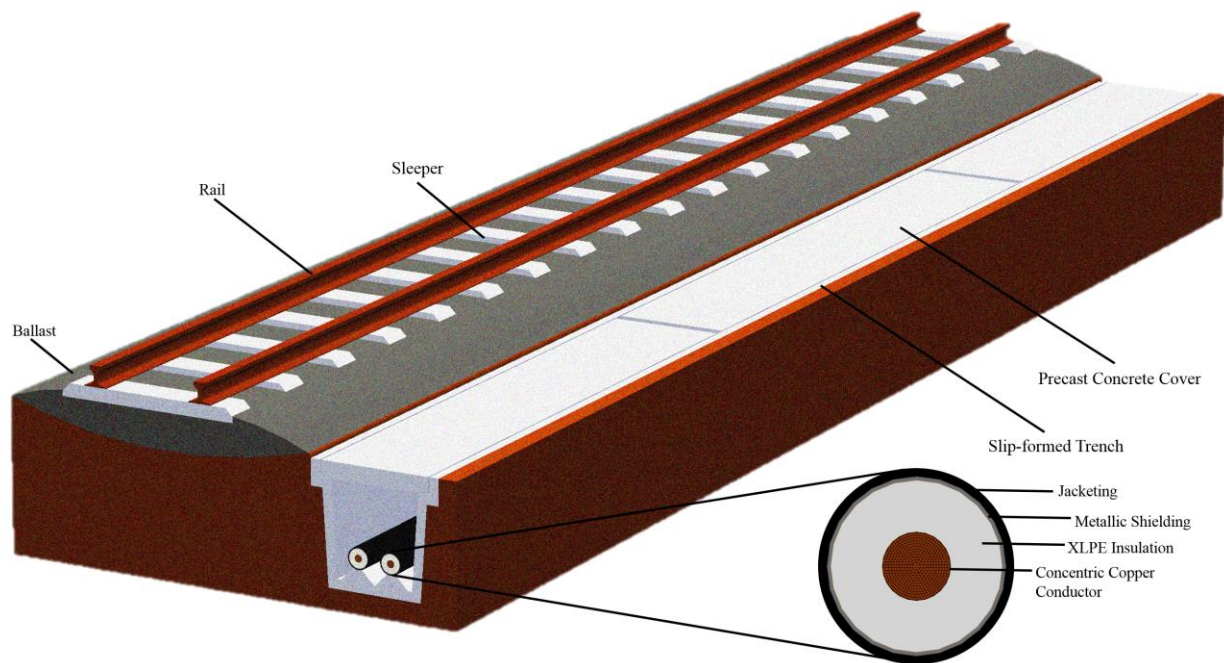
Figure 8: An example of a UGC system located next to railroad tracks. The bipole cable configuration is housed inside of a slip-formed concrete duct bank and covered with precast concrete slabs. Heat transfer analysis and simulation concluded that compacted backfill, which could comprise native soil, would be necessary to prevent overheating of the cable cores.
