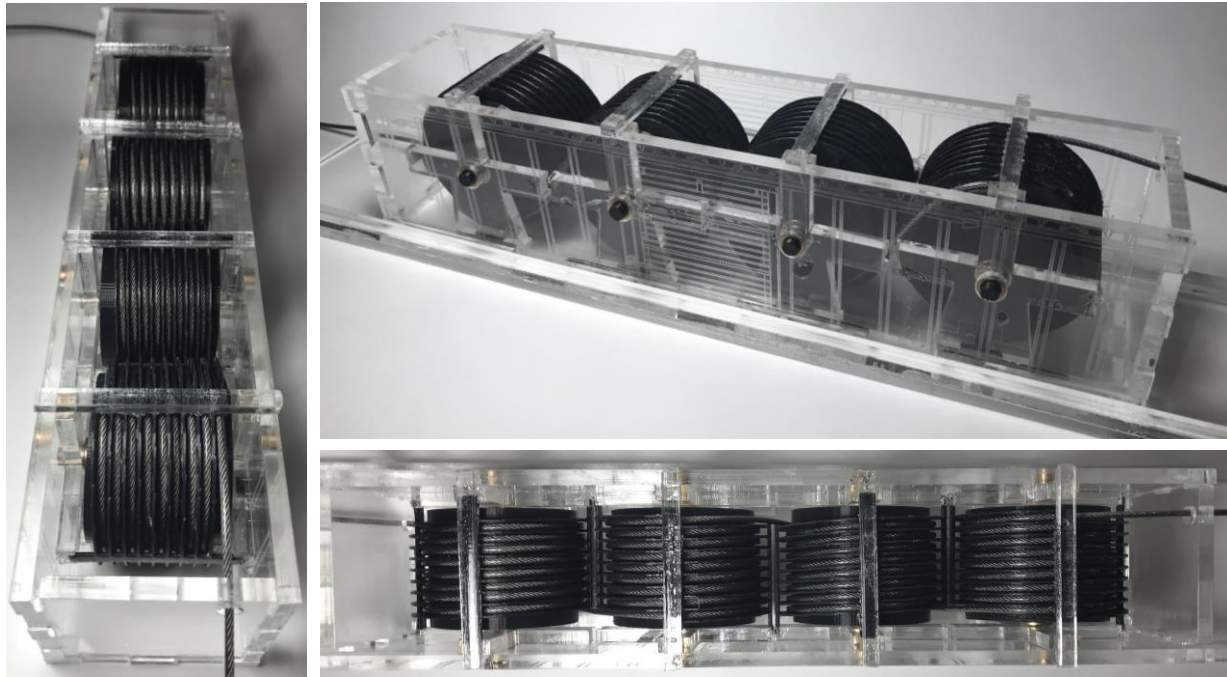
Figure 7: A 50:1 scale model of a concept for a “degassing train” capable of greatly increasing the amount of cable in a series of railcars while continuously processing it as the train moves relative to it in an inertial reference frame. The cable proceeds down the length of the train by passing from reel to reel, moving axially across the length of each reel under the influence of non-rotating helical guides. According to an analytical model, the bending, tension, side-wall pressure, and accumulated twist in the cable are safe. This accomplishes approximately a 40x decrease in the length of the degassing section of the train.
