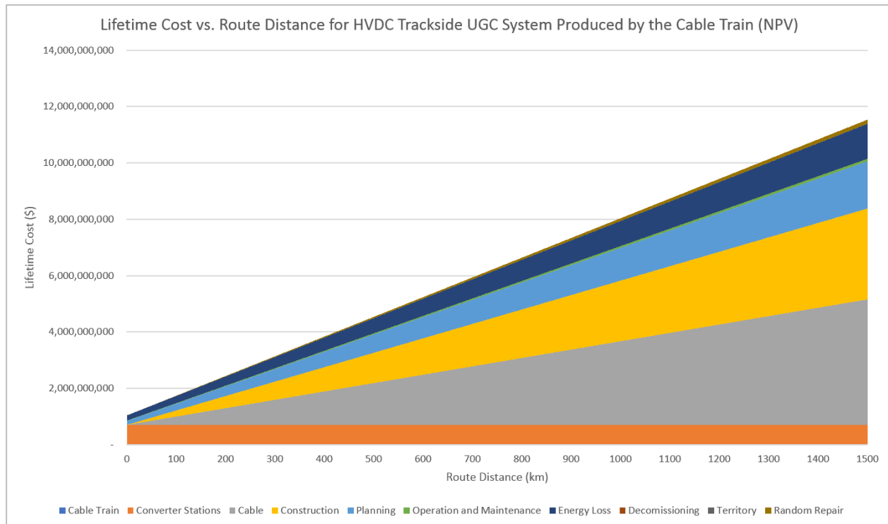
Figure 11: The estimated lifetime cost of a trackage HVDC UGC system produced using the Cable Train, broken down into gross cost categories. Cost of the Cable Train itself is small compared to other capital costs.
