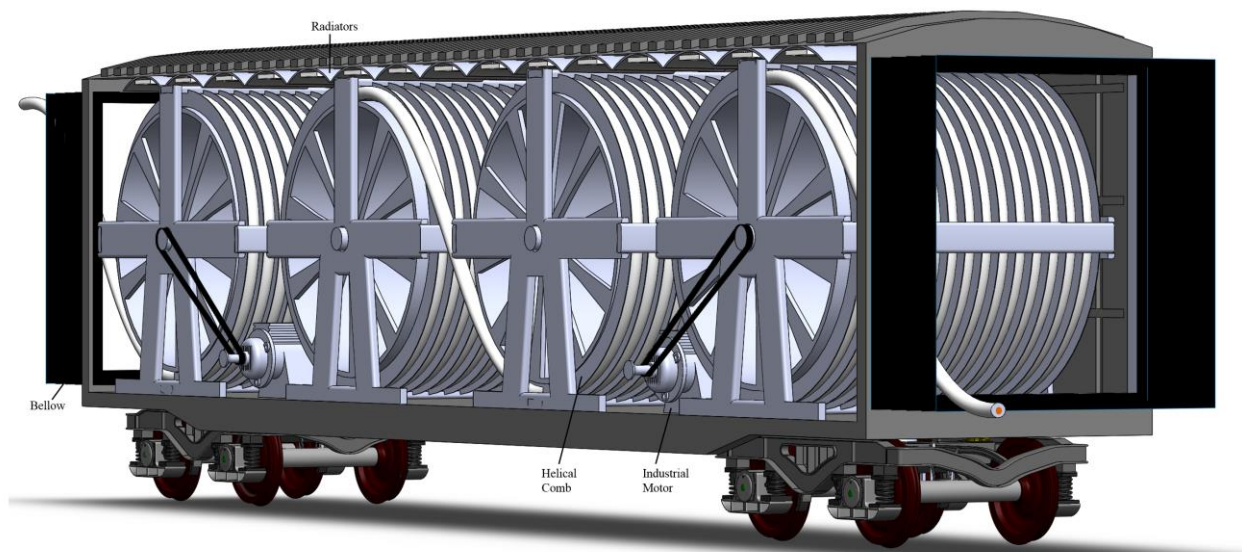
Figure 4: Illustration of an inline cable handling system concept that increases the length of cable that can safely fit into a single boxcar, thereby decreasing the number of cars that are needed to sufficiently degas cable after insulation extrusion. On each reel, the cable travels across the width of the railcar/container, alternating direction with each reel. Helical guides are used to guide the cable across each reel and overhead radiant heaters provide the heat necessary to expedite the degassing process.
