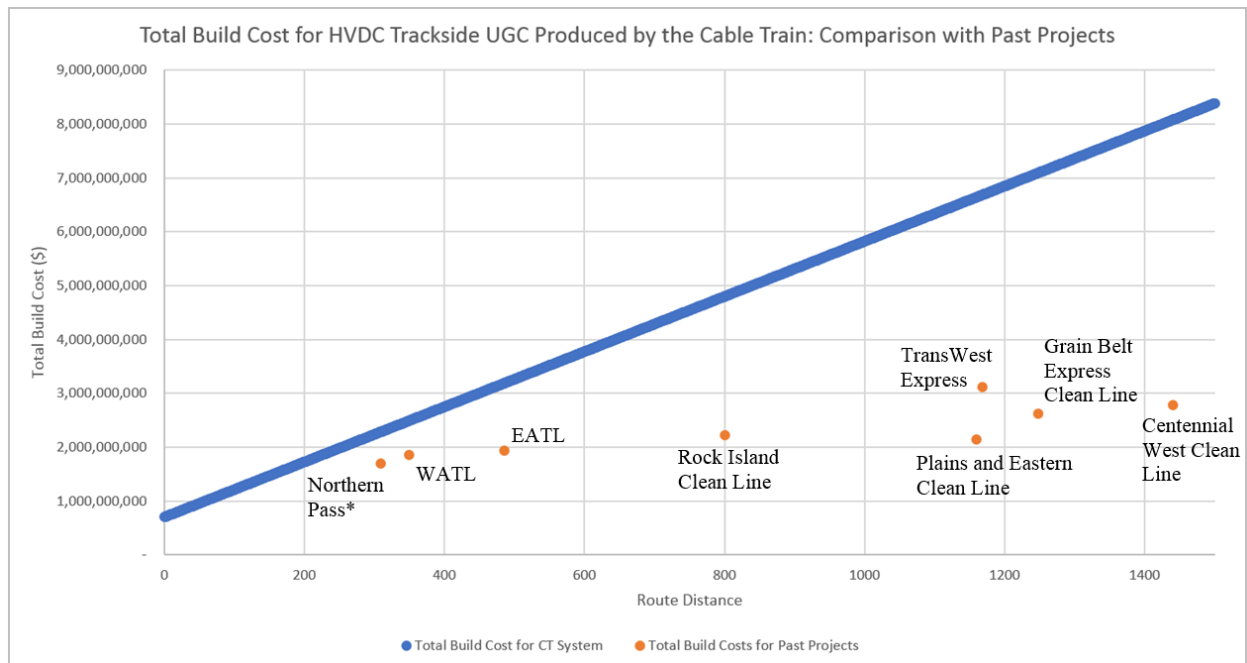
Figure 12: The estimated build cost of a trackage HVDC UGC system produced by the Cable Train, graphed alongside the self-reported, projected build costs of other HVDC projects [27], [33]-[39]. *Northern Pass is no longer being pursued due to regulatory delays.
