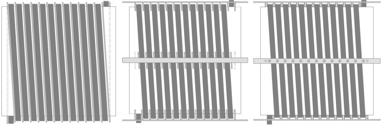
Figure 5: Schematics of a continuous helical comb (Left, a), discrete “fin” comb (Middle, b), and a discrete roller comb (Right, c) that ensure the cable moves axially down the length of the drums.
