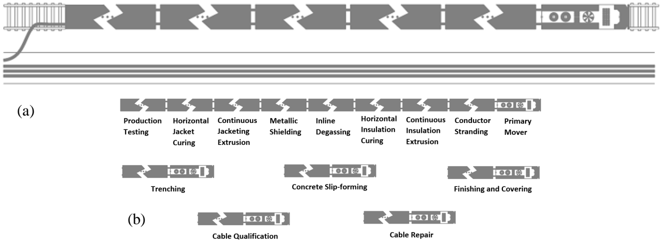
Figure 2: (a) Plan view of the “Cable Train,” which lays in-situ produced high voltage cable into an adjacent, open trench. The train comprises a number of modules necessary to manufacture high voltage cable – wire stranding, extrusion, curing, and degassing, among others. (b) A diagram showing the possible separation of Cable Train functional units. Each of these modules may be independently hauled in order to fully realize the maximum working speed of each module.
