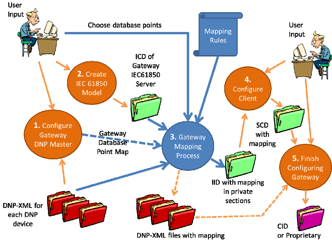
Figure 5 Use Case B Mapping Steps
