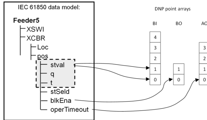
Figure 2 IEC 61850 Attribute Mapping
