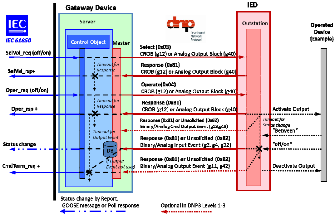
Figure 7 SBO With Enhanced Security (Use Case B)
