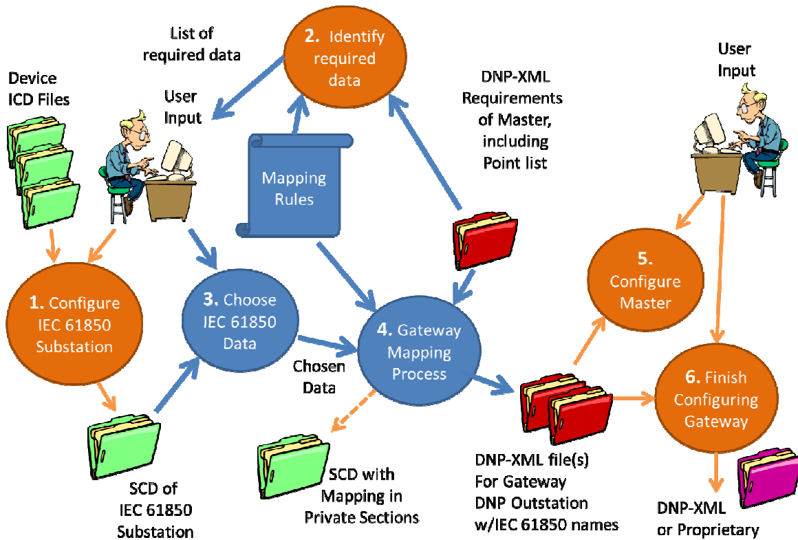
Figure 4 Use Case A2 Mapping Steps
