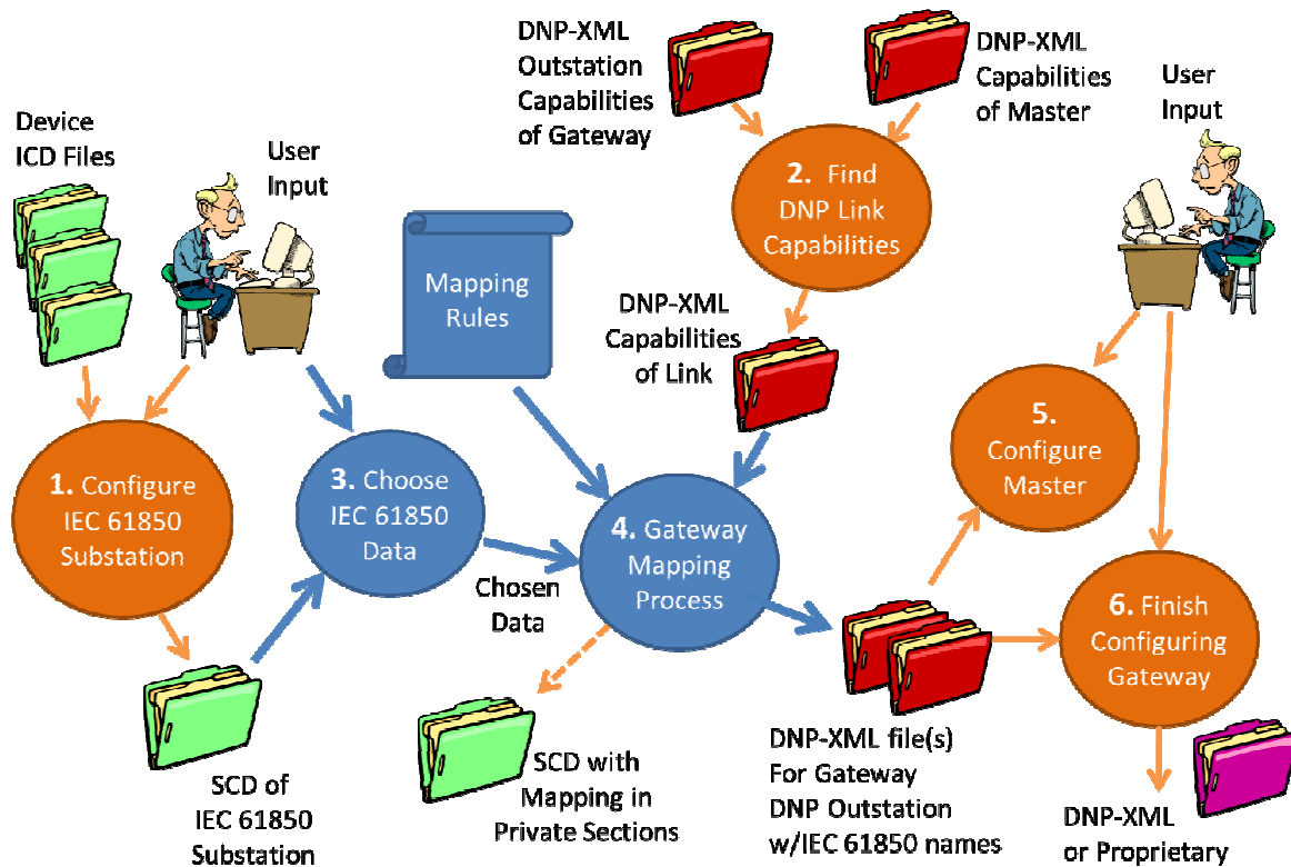
Figure 3 Use Case A1 Mapping Steps
