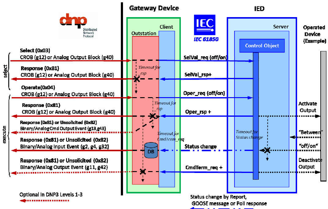
Figure 6 SBO With Enhanced Security (Use Case A)
