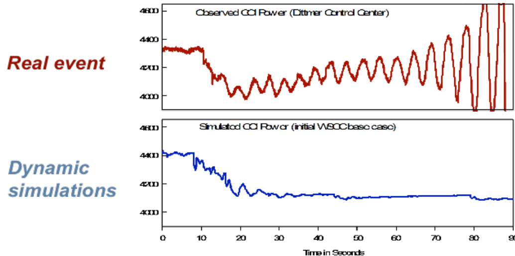
WSCC August 1996 outage – real versus simulation
